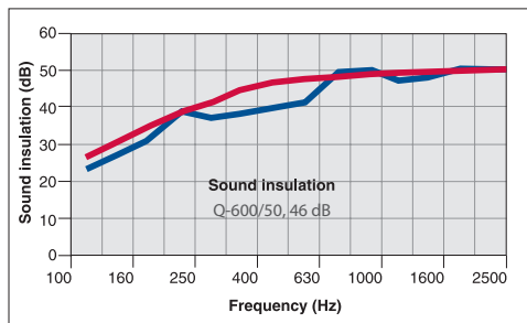
— Adjusted References — Sound Reduction Index (Laboratory measurement)
